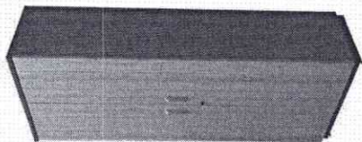
Armário Extra Alto 2 Portas BEL-AX001 | 800X450X2000 BEL-AX002 | 800X500X2000 BEL-AX003 | 900X450X2000 BEL-AX004 | 900X500X2000
